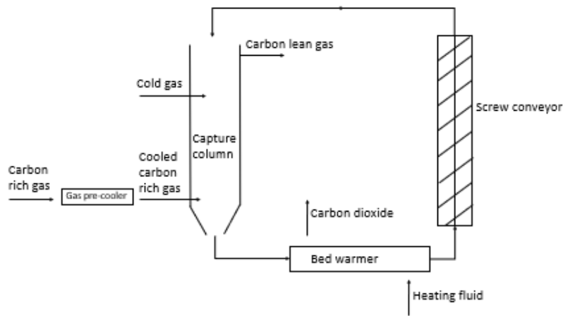
Figure 1. Sketch of proposed design
