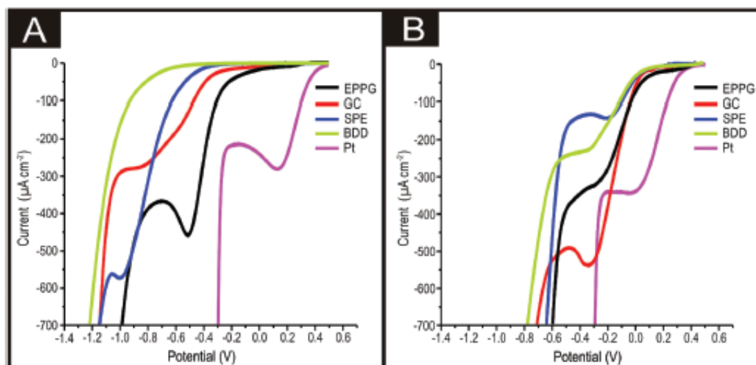
Fig. 1 (A) LSVs of bare/unmodified EPPG, GC, SPE, BDD and Pt electrodes showing signals corresponding to the ORR. (B) LSVs recorded using 1524 \text{ ng cm}^{-2} 2\text{D-MoS}_2 modified EPPG, GC, SPE, BDD and Pt electrodes showing the position of ORR peaks. In all cases; scan rate: 25 \text{ mV}^{-1} \text{ s}^{-1} (vs. SCE) and a solution composition of 0.1 M \text{H}_2\text{SO}_4 which is oxygen saturated.
