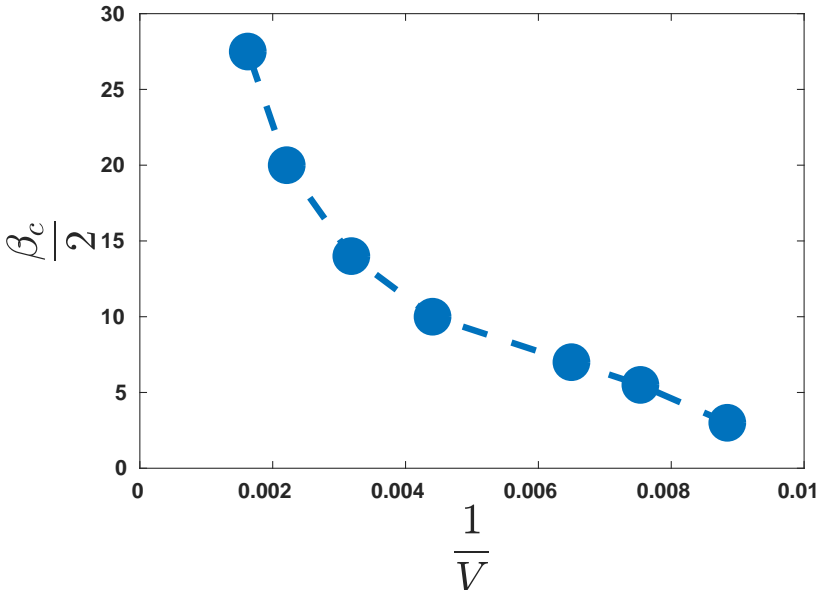
Figure 13. Critical sensitivity with respect to the inverse capacity of the IBM over 5 simulations. Throughout the simulations, we kept the total density at 0.2 and the total number of cells was 500.
