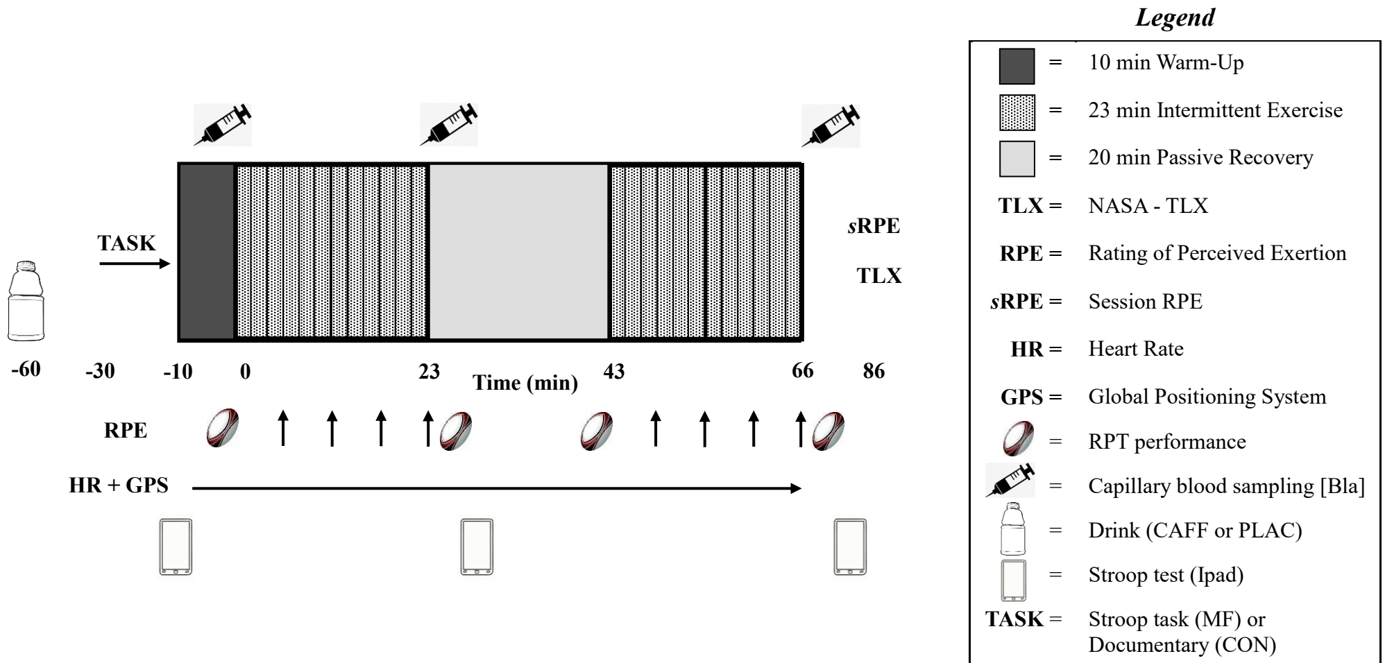
Figure 6.1. Schematic of the rugby league movement simulation protocol, including measurements. NASA-TLX = subjective task load index; RPT = rugby passing test; [Bla] = blood lactate concentration; CAFF = caffeine drink ( 5 \text{ mg}\cdot\text{kg}^{-1} ); PLAC = placebo drink; MF = mental fatigue trial; CON = control trial.
