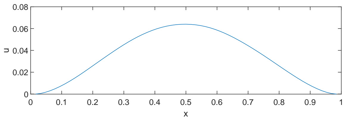
Figure 5.7.6: Approximate realisation of the solution at time T = 1 with \alpha = 1.5 and \gamma = 0.9 in Example 55
