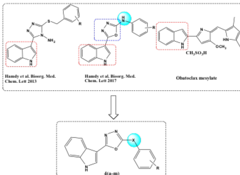
Figure 1. Rational design of novel indole-based oxadiazoles 4a–m .
