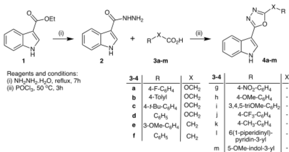
Scheme 1. Synthesis of 2-(1H-indol-3-yl)-5-substituted-1,3,4-oxadiazoles 4a–m .
