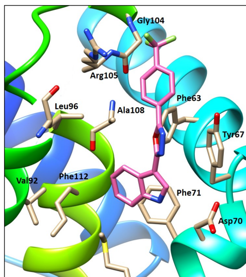
Figure 3. Compound 4j showed hydrophobic interactions with key residues Tyr67, Phe71, Leu96 and Ala108, in addition to a p-cation interaction between the trifluorophenyl group and the key residue Arg105.
