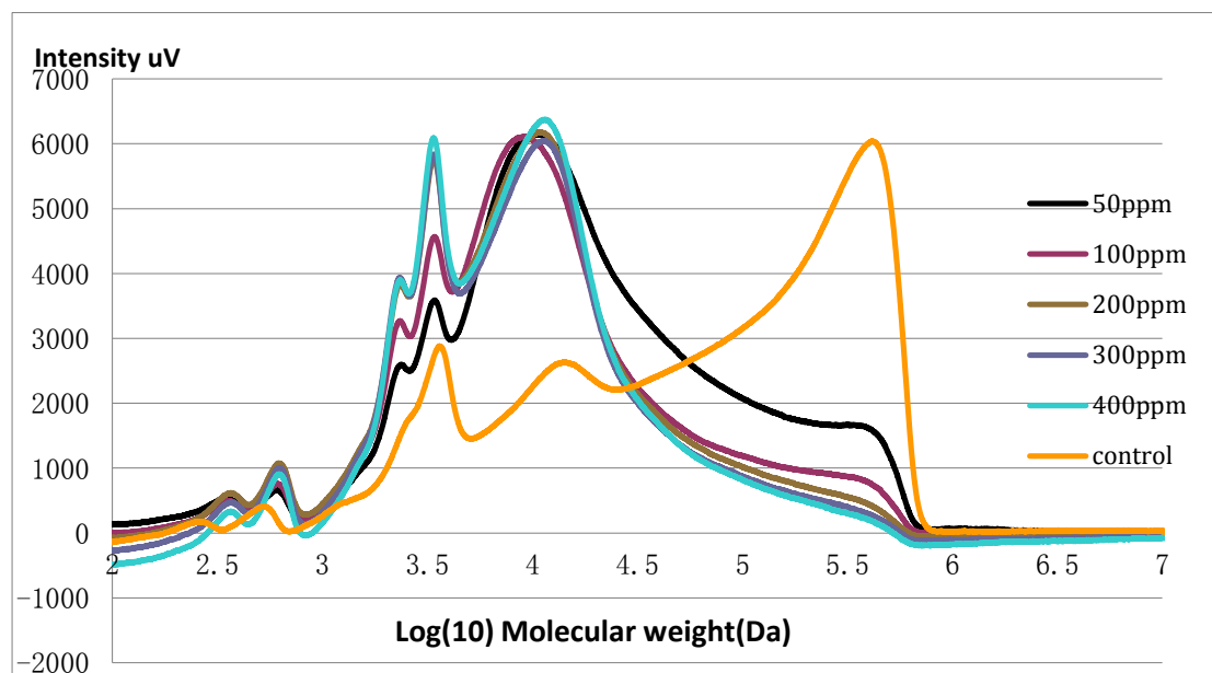
Figure 1. The molecular weight distribution of E-WEAXs with enzyme treatment of various concentrations
