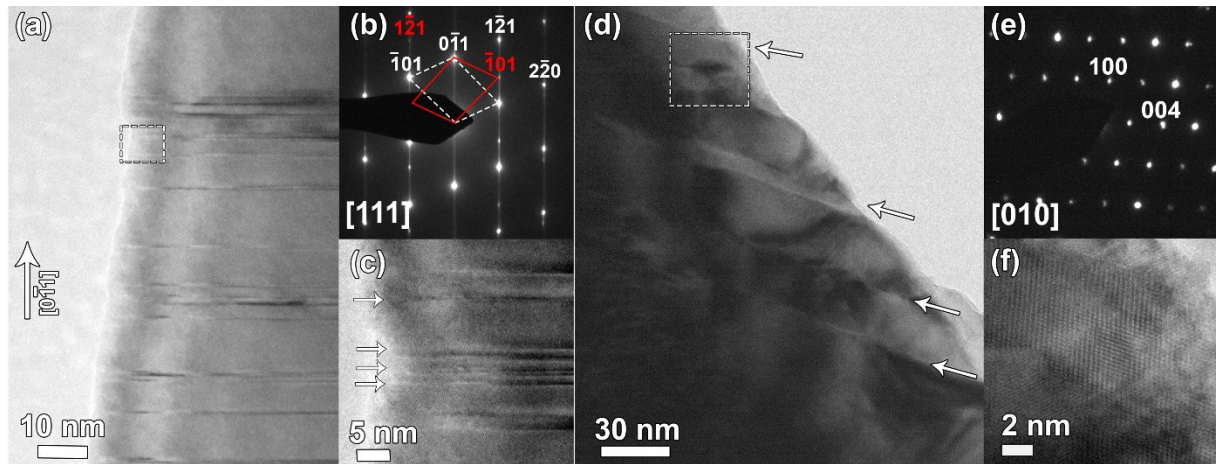
Figure 3 (a) HRTEM image of defects in CS1250; (b) selected area diffraction pattern (SAED) taken from the crystal in (a). Red and white indices indicate reflections on the SAED that are coming from different twin domains in the rutile structure; (c) HRTEM image of the area marked by dashed lines in (a), showing twin defects; (d) bright-field electron microscopy image showing complex defects in CS1250. White arrows indicate positions of faults; (e) SAED pattern taken from the area of the crystal with defects shown in (d). The pattern is indexed in the \text{Ti}_4\text{O}_7 Magnéli phase. (f) HRTEM image of the area marked by dashed lines in (d), showing the \text{Ti}_4\text{O}_7 Magnéli phase area of the grain.
