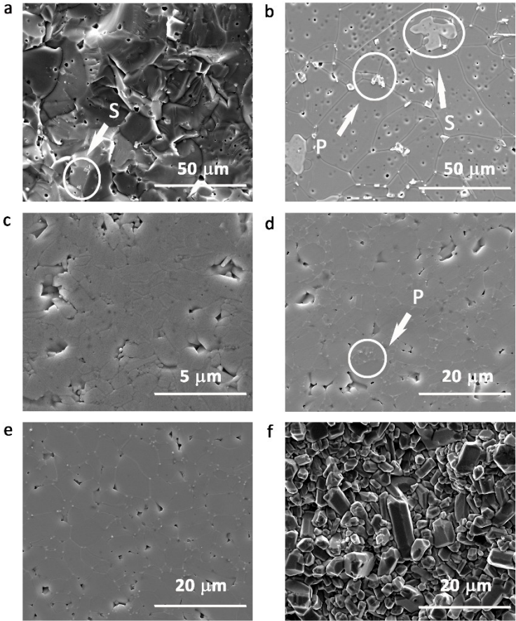
Figure 1 SEM of (a) fracture surface of CS1210; (b) CS1210 thermally etched at 1150 °C; (c) SPS1050 thermally etched at 1000 °C; (d) SPS1200 thermally etched at 1050 °C; (e) SPS1250 thermally etched at 1100 °C; (f) fracture surface of SPS1250 (S denotes sintering aid; P, precipitation)
