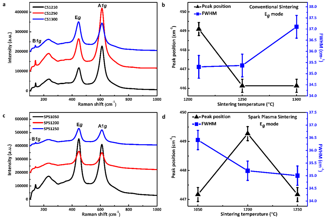
Figure 4 (a) Raman spectra of conventional sintering samples; (b) peak position and FWHM of the Eg mode of CS samples; (c) Raman spectra of SPS samples; (d) peak position and FWHM of Eg mode of SPS samples.
