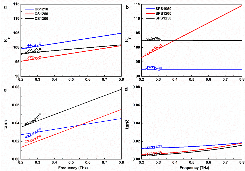
Figure 5 Frequency-dependence of (a) permittivity in CS samples; (b) permittivity in SPS samples; (c) dielectric loss in CS samples and (d) dielectric loss in SPS samples in the THz sub-spectral domain (0.20 - 0.80 THz). The solid lines are the experimental results from THz-TDS system and the discrete points are the experimental results from the VNA+QO transmission system.
