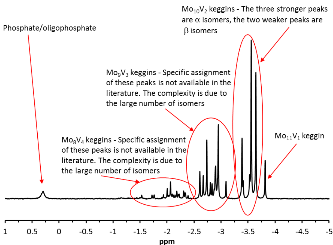
Figure S5. ^{31}\text{P} spectrum for a fully oxidised (i.e. 100% vanadium(V)) sample of 0.3 M \text{H}_6\text{PV}_3\text{Mo}_9\text{O}_{40} at 298 K.
