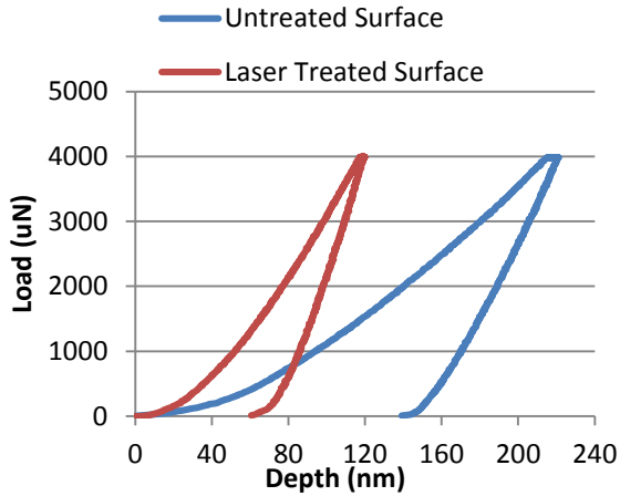
Figure 3. Nano-indentation curves of the treated and untreated samples
