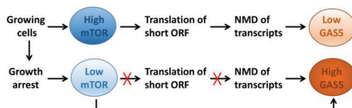
Figure 2. Interplay between mammalian target of rapamycin (mTOR) and nonsense-mediated decay (NMD) regulates cellular GAS5 lncRNA levels.
